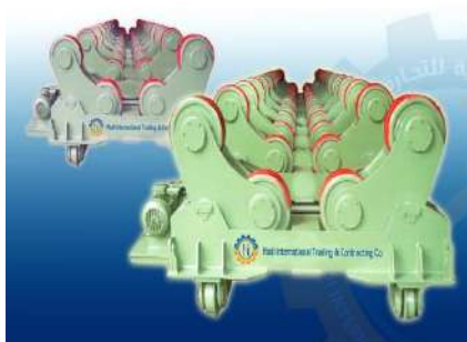
Welding Rotators
